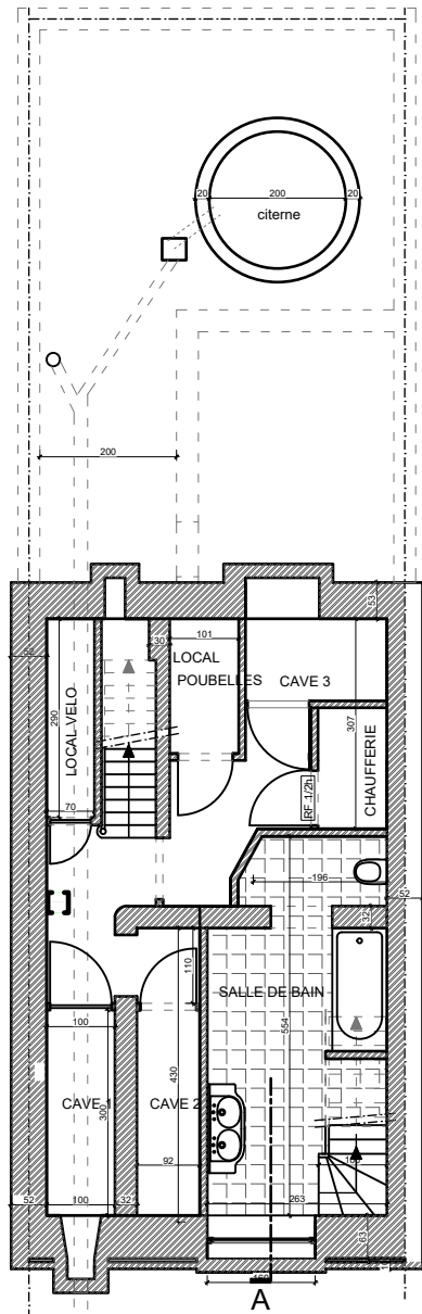
CAVES - PROPOSES
