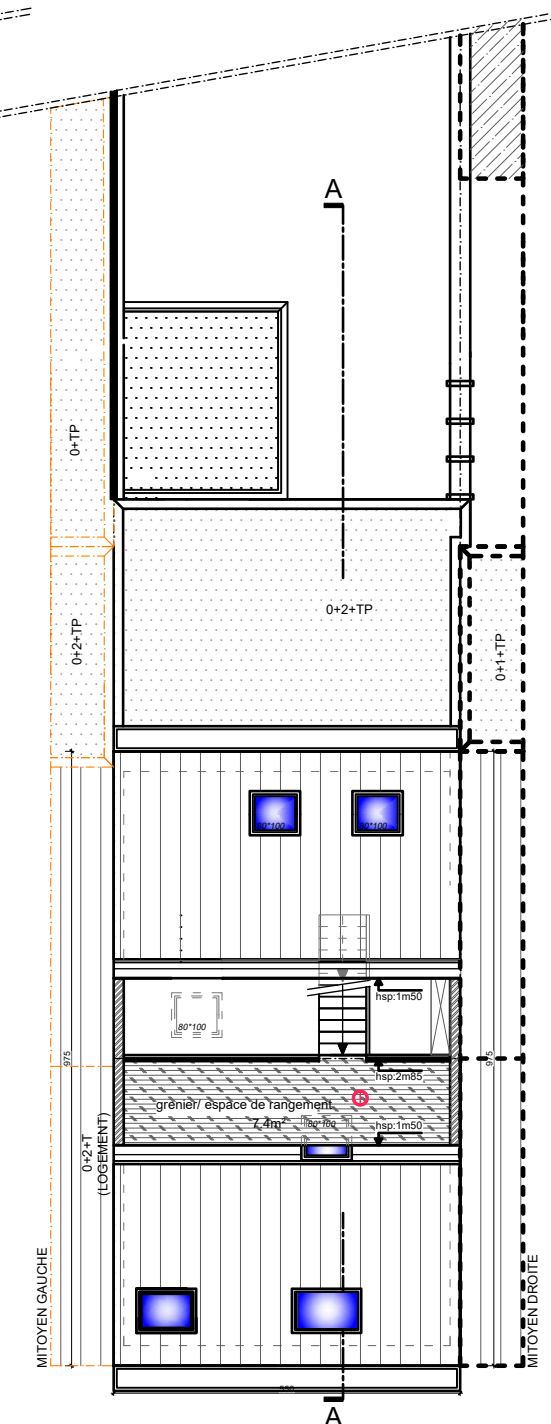
MEZZANINE - PROPOSES
