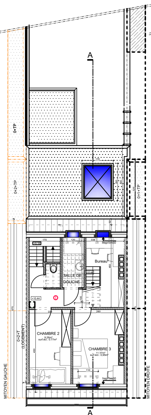
COMBLES - PROPOSES
